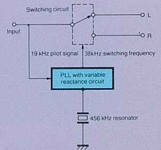
Fig. 5 Stereo Demodulator of the T-11
