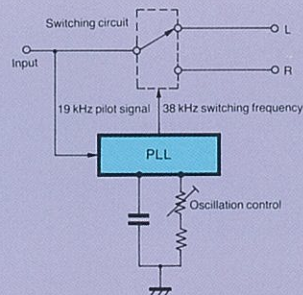
Fig. 4 Trimmer Potentiometer Type Stereo Demodulator
